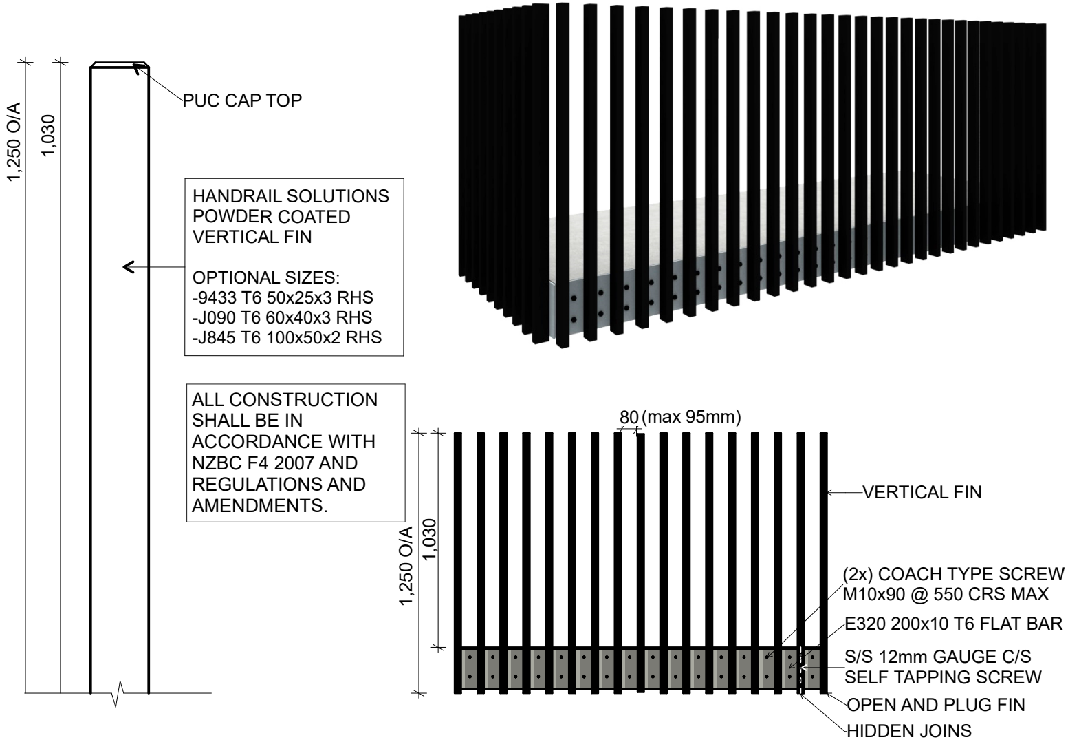
BALUSTRADE SECTION SCALE 1:5 @ A4
